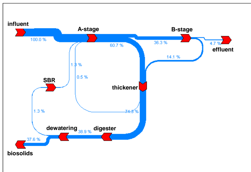
Figure 4. Simulated COD-balance of the WWTP Strass based on a 2 weeks measurement campaign in summer 2004 (average load 119866 PE 120COD ; average flow 23771 m 3 /d; Temperature 16.8°C).
