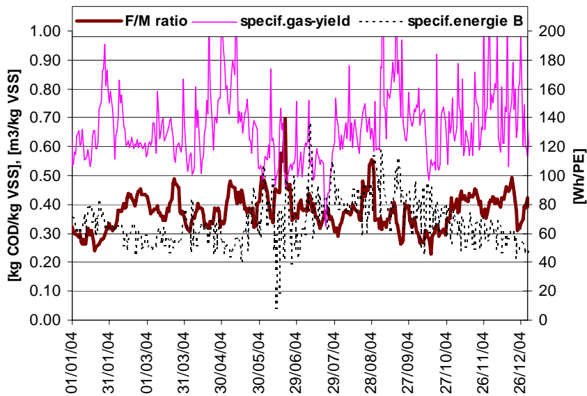
Figure 5. F/M ratio in [kg COD per kg aerobic VSS] is plotted against specific aeration energy demand and the biogas yield.
