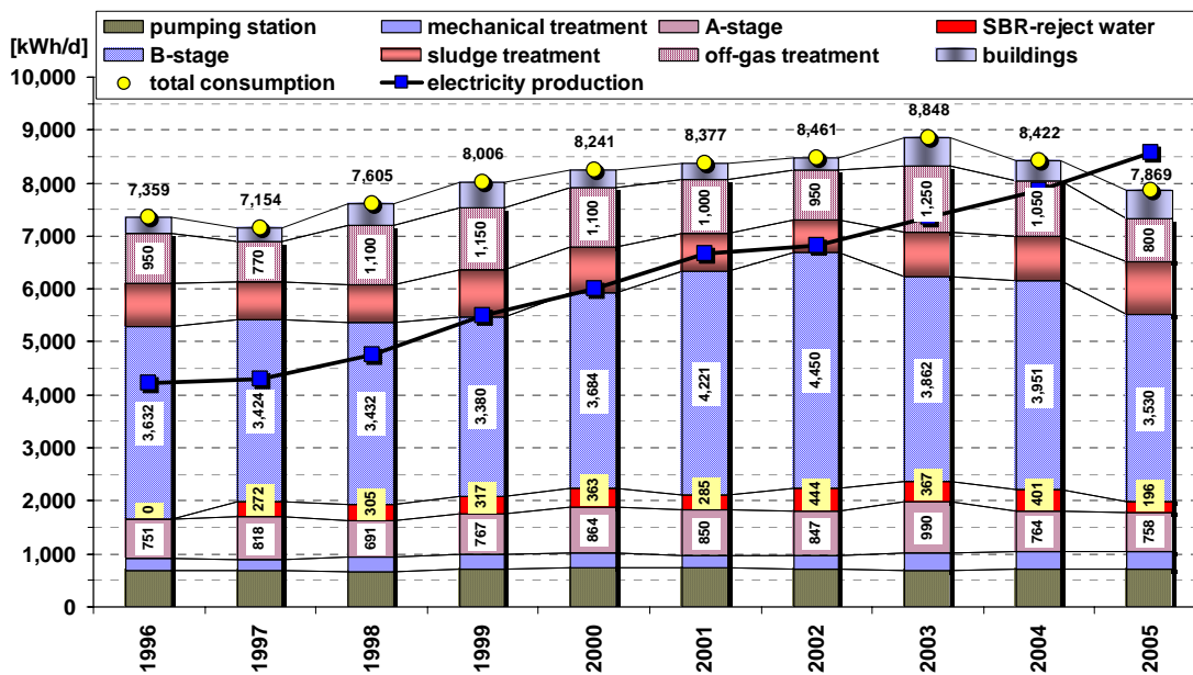
Figure 7. Energy demand of individual unit processes of the WWTP Strass.
