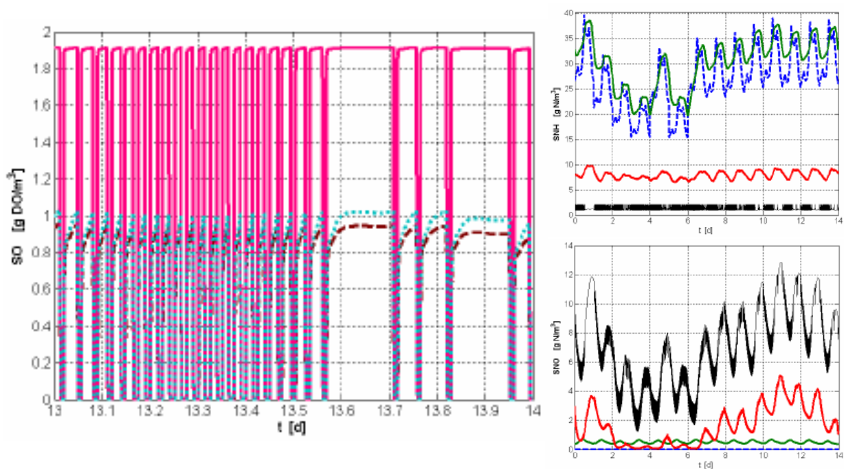
Figure 6. Simulated DO-profile during one day of on-line ammonia controlled intermittent aeration and dynamics in ammonia and nitrate concentrations during a 14 days run.
