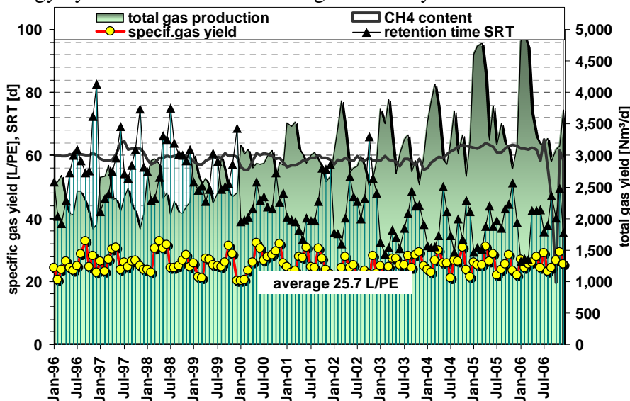
Figure 8. Specific biogas yield and methane content in correlation with retention time.
